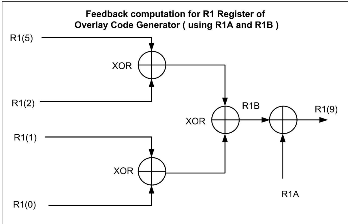
Figure 15: R1 Register feedback computation for overlay codes
