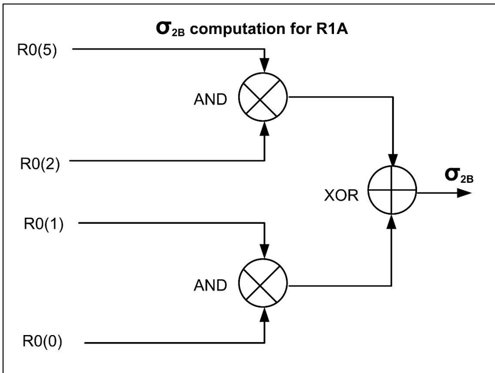
Figure 14: \sigma_{2A} and \sigma_{2B} computation for overlay codes
