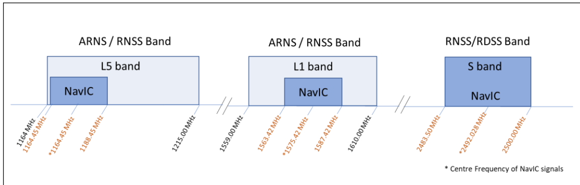
Figure 3 :Frequency bands of NavIC Signals
