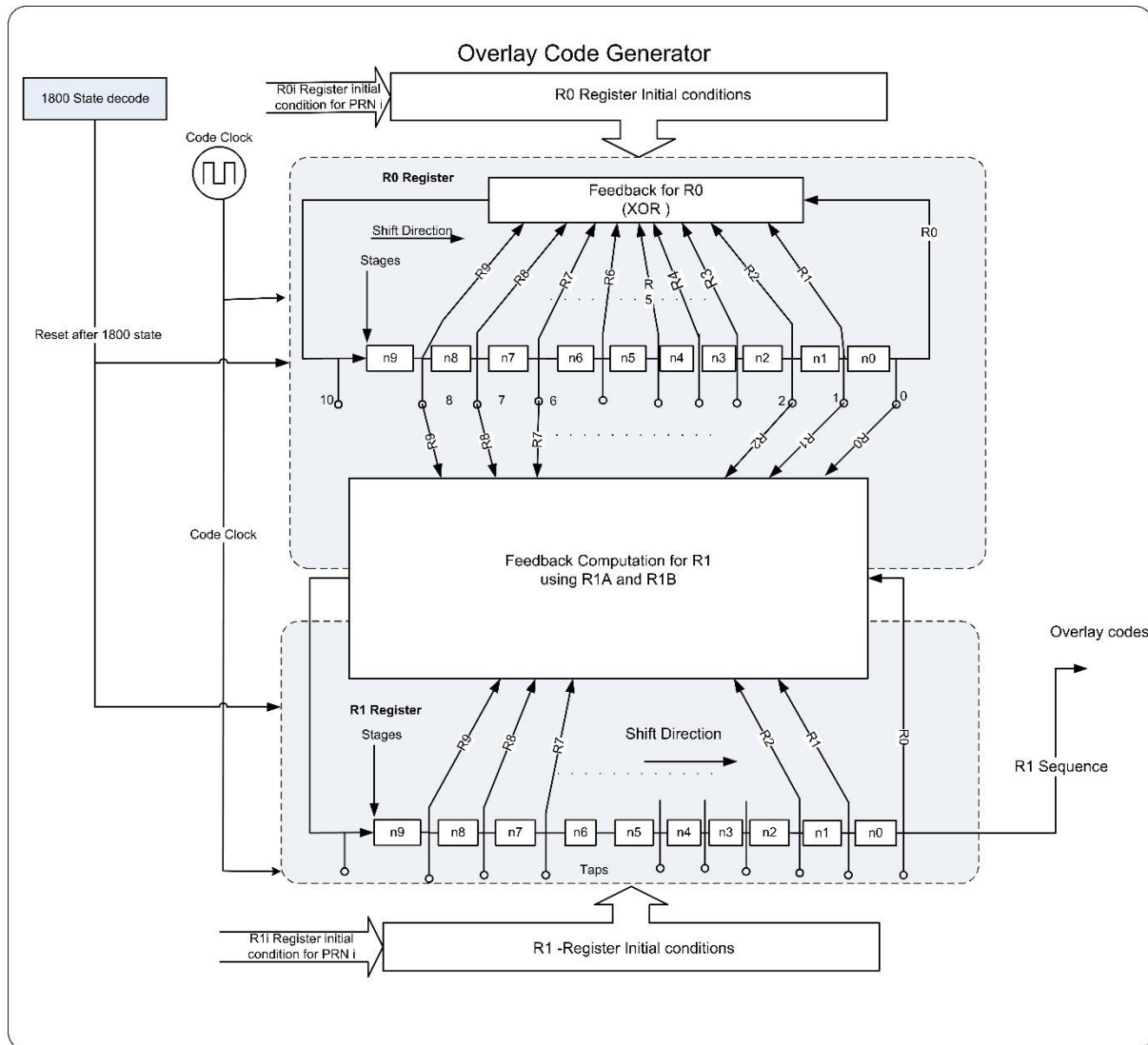
Figure 12: Block Diagram of overlay sequence generator
