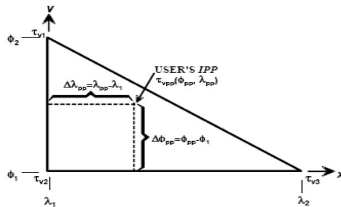
Figure 27: Three Point Interpolation Algorithm
