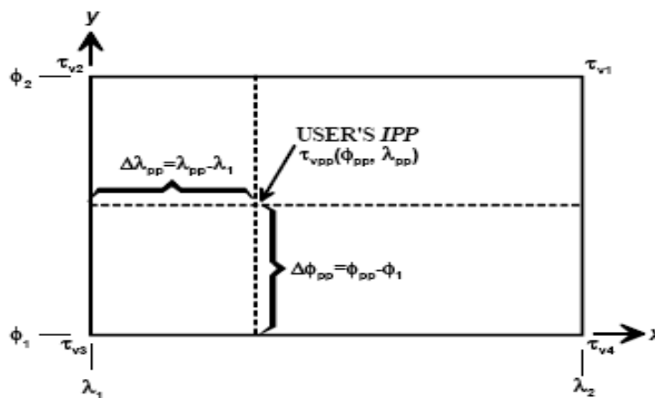
Figure 26: Four Point Interpolation Algorithm
