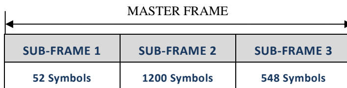
Figure 19: Master Frame Structure
