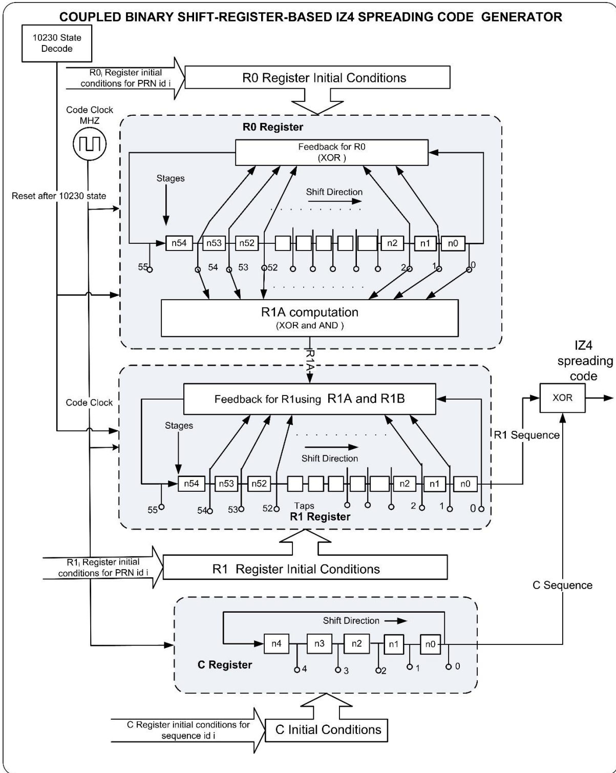
Figure 6: Functional Description of IZ4 Sequence generation using Binary shift registers.
