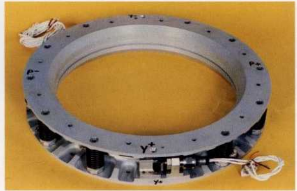
KITSAT - 3 separation system
