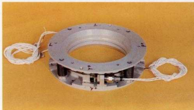
TUBSAT Separation System
