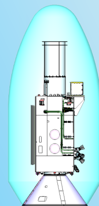
Encapsulated Assembly
